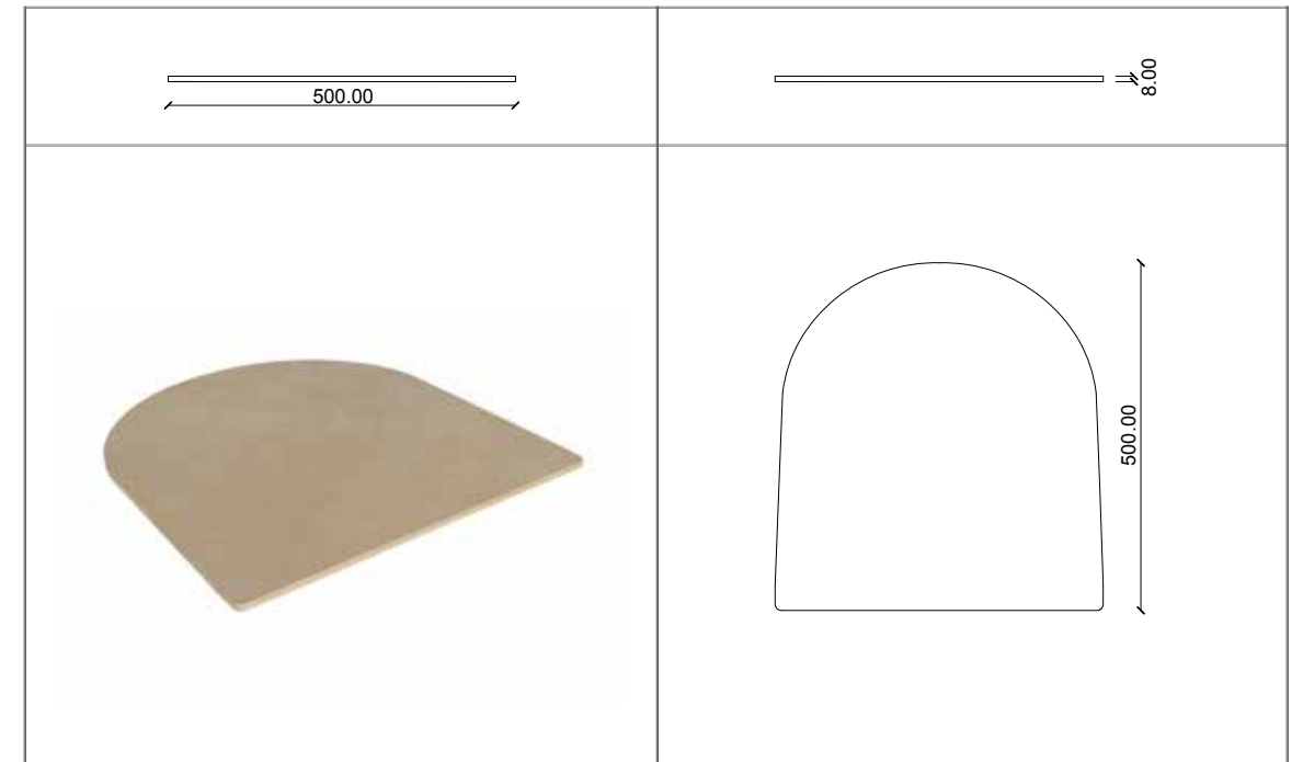
HUNKAR - IRIS 10 - 20 - 30 / SEAT
