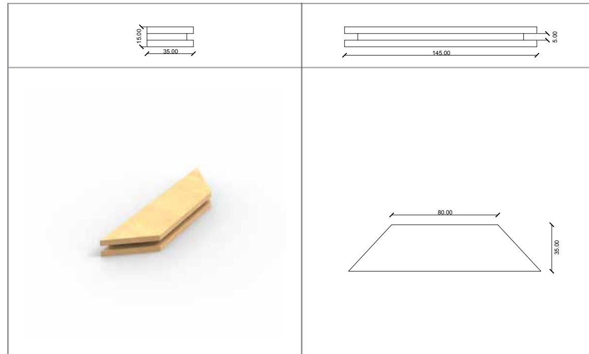
HUNKAR - IRIS 10 - 20 - 30 / CORNER SUPPORT
